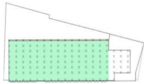
Gambar 7. Denah Eksisting Lantai 2
