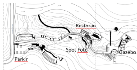
Gambar 10. Masterplan Bangkiang Jaran Waterfall
