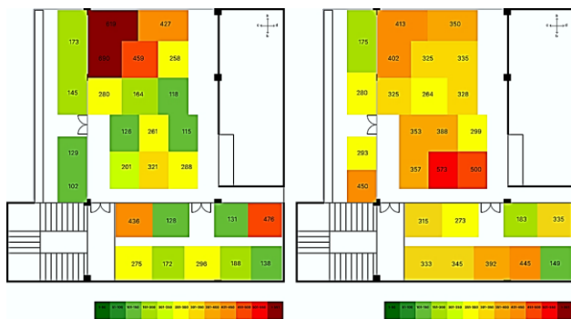
Figure 7. Illuminance level measurements during daytime (left) and nighttime (right) in Cafe A
