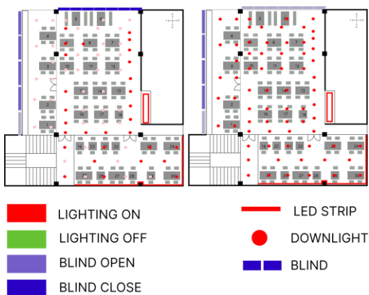
Figure 4. Luminaire condition daytime (left) and nighttime (right) in Cafe A
