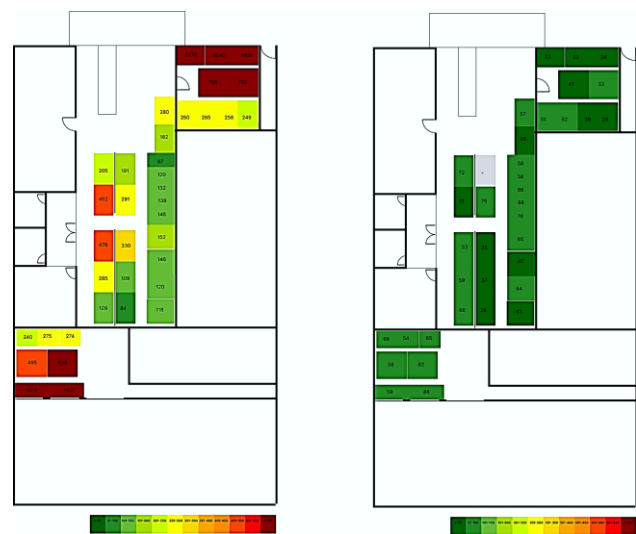
Figure 10. Illuminance level measurements during daytime (left) and nighttime (right) in Cafe B
